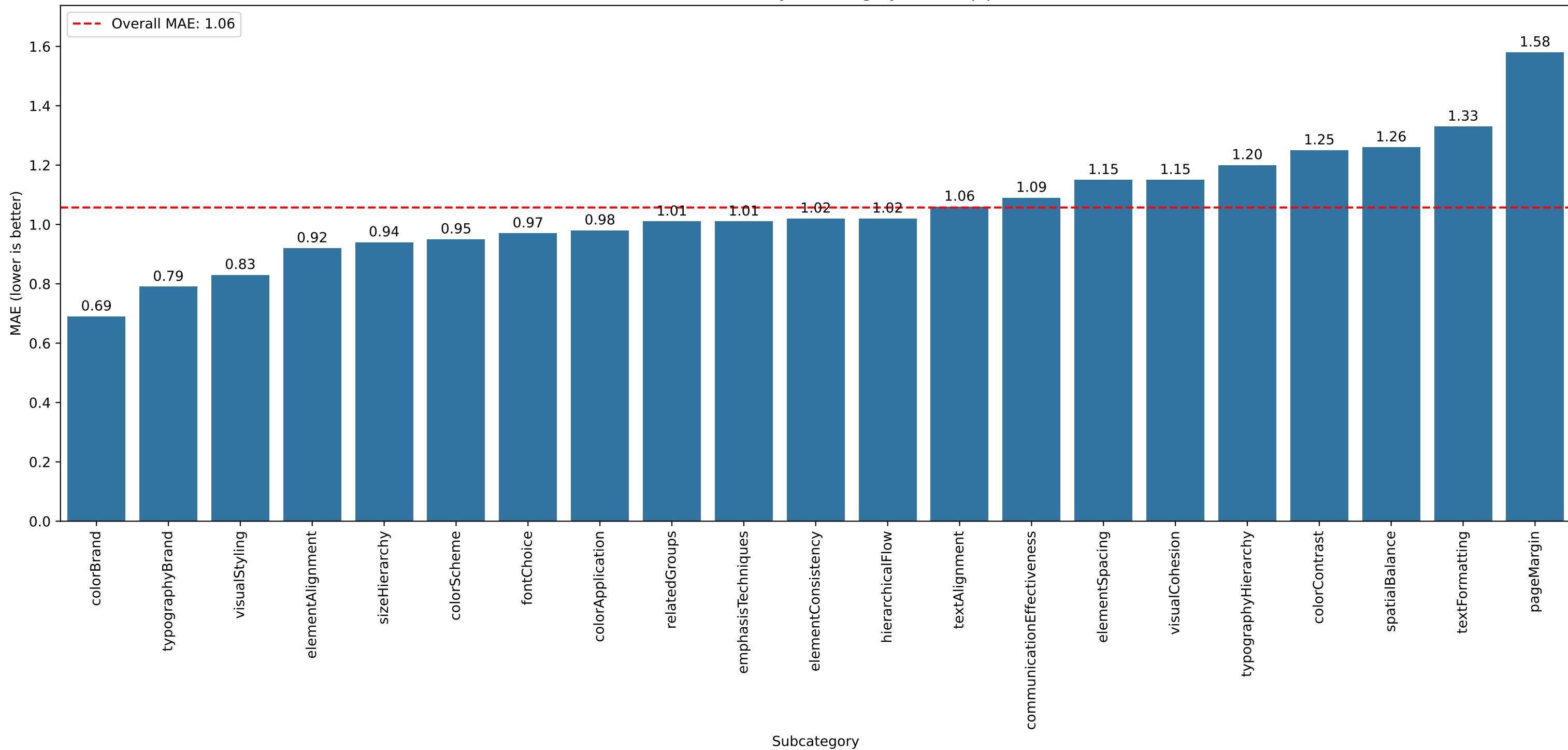
Mean Absolute Error by Subcategory: llama3-pipeline
