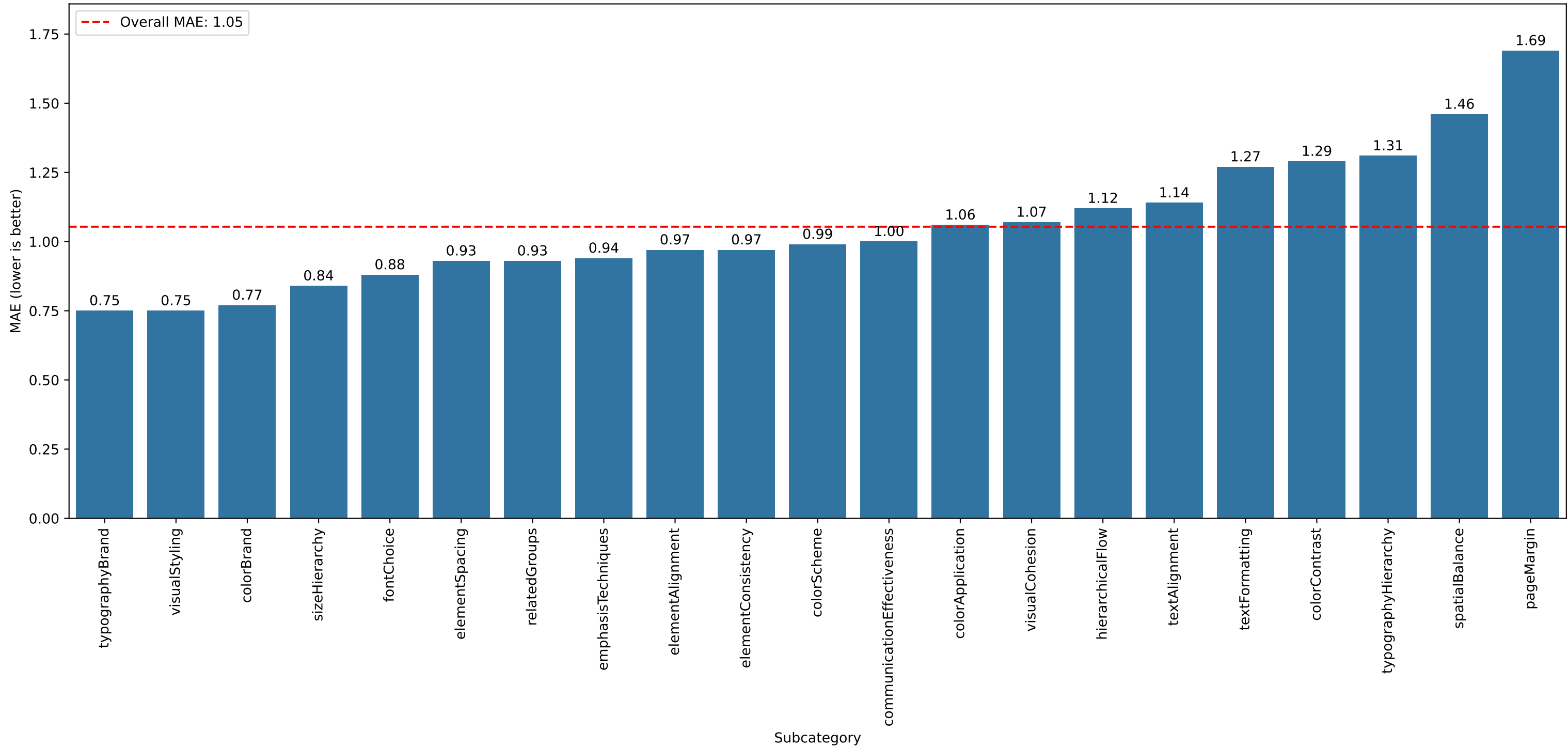
Mean Absolute Error by Subcategory: Llama-4-Scout-17B-16E-Instruct-FP8
