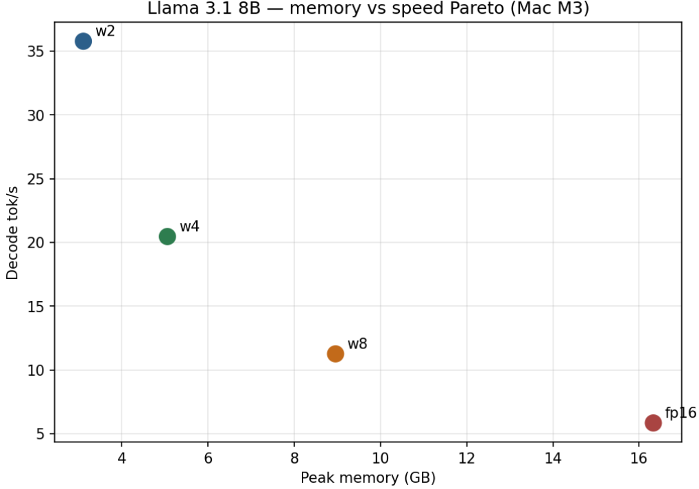
Figure 6: Memory–speed Pareto across weight bit-widths and models. Moving from FP16 to 4-bit is a joint win on both axes for bandwidth-bound decode—the difference between “science fair” and “I leave this running all day.”
