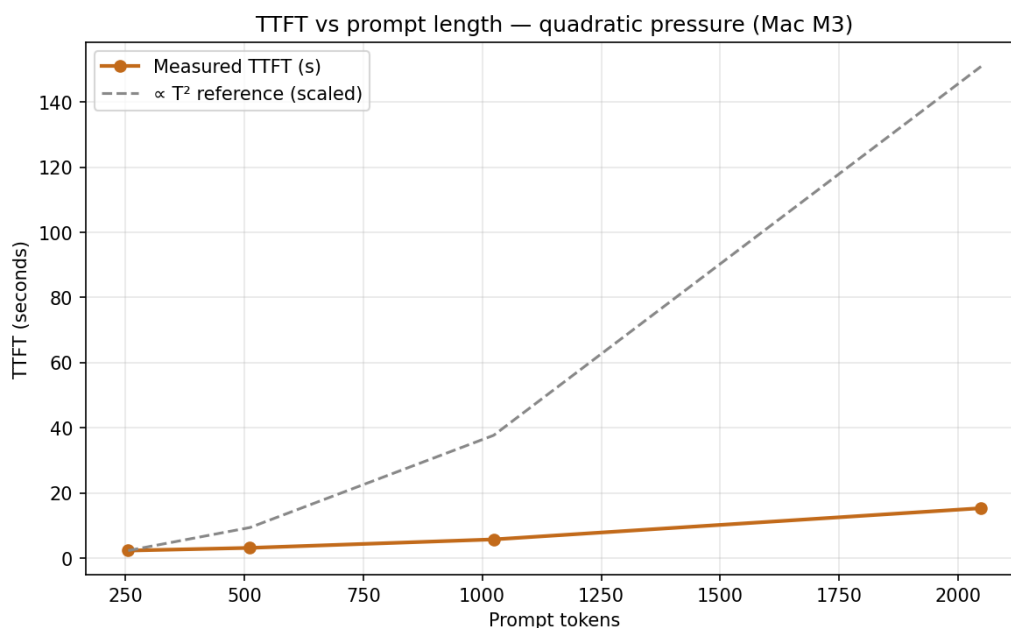
Figure 9: TTFT versus prompt length. Local RAG dies in prefill, not in the tokens/s column. Everyday-device UX is a prefill SLO.
