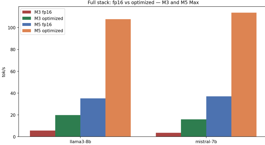
Figure 7: Same software stack, two chips. Relative wins from leaving FP16 travel; absolute UX does not: \approx 20 tok/s on M3 is usable chat, \approx 100+ tok/s on M5 Max makes the UI the bottleneck.
