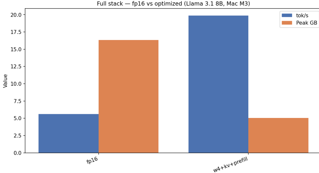
Figure 10: Mac M3, Llama 3.1 8B: FP16 versus the stacked 4-bit + KV + prefill recipe. Memory falls to \approx 31\% of baseline; decode rises \approx 3.55\times —enough that the machine remains a daily-use computer.
