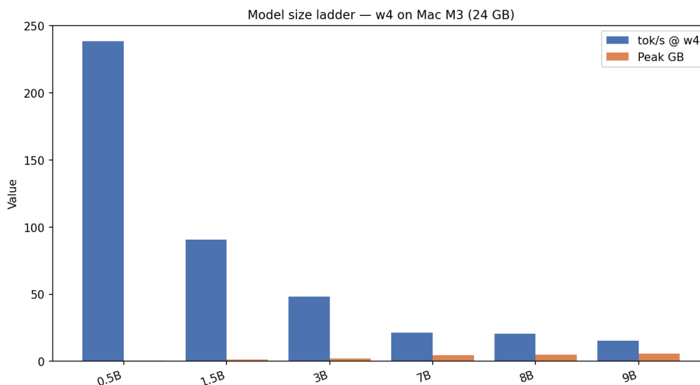
Figure 8: Dense 4-bit model ladder on Apple Silicon. Size is an inference optimization: quality, memory, and tokens/s move together.
