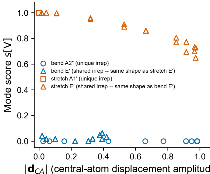
(a) Trigonal-planar AB_3 (non-ideal)
