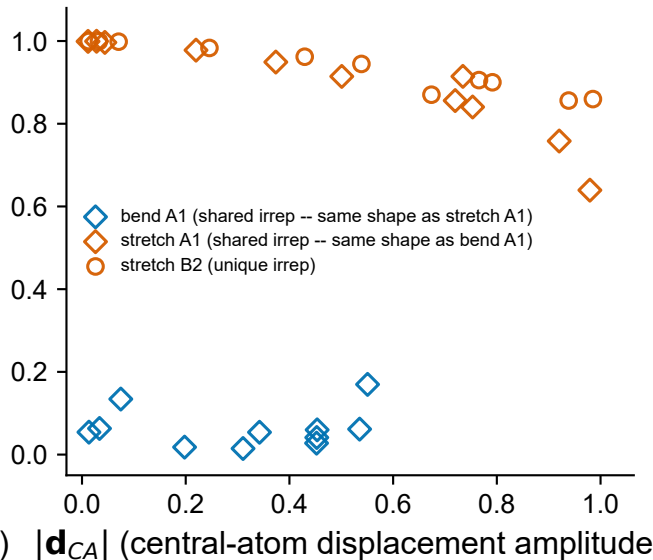
(b) Bent AB_2 (non-ideal)
