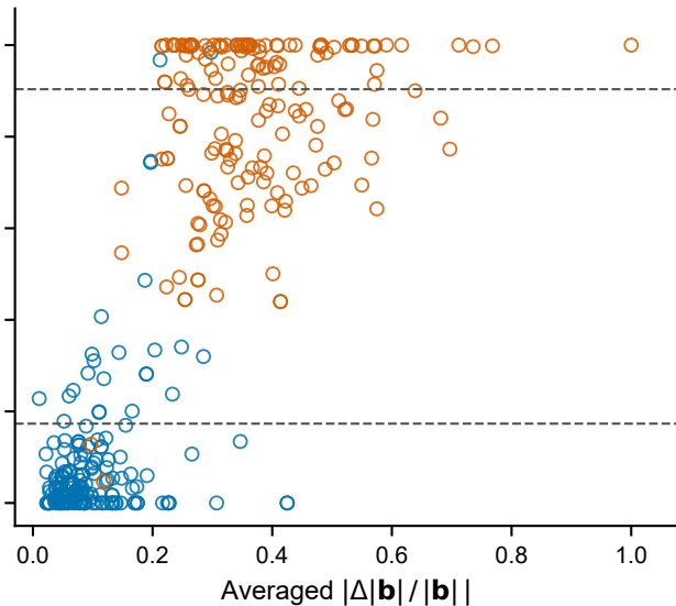
(b) Non-ideal molecules
