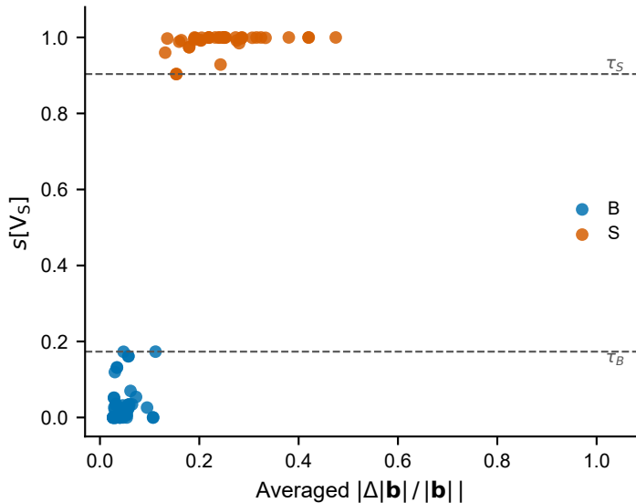
(a) Ideal molecules
