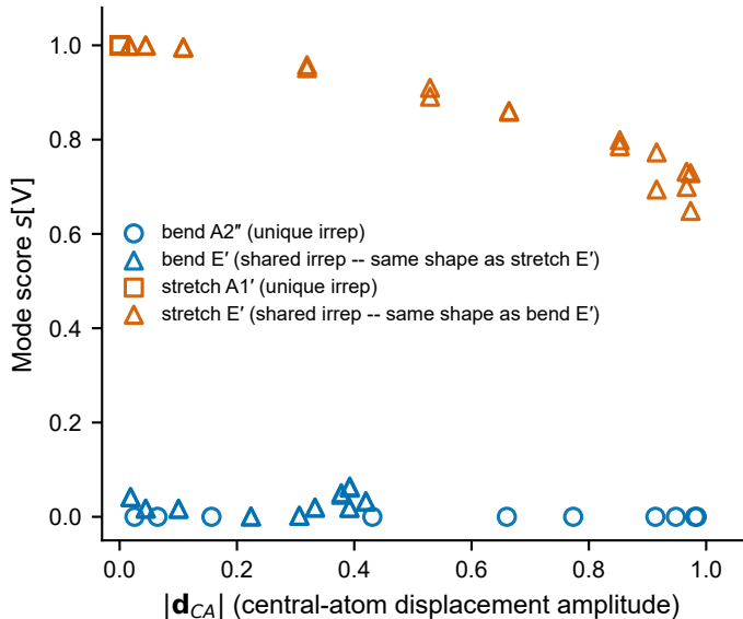
(a) Trigonal-planar AB_3 (non-ideal)
