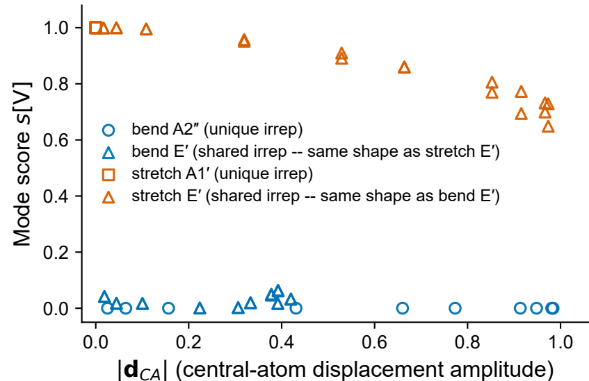
(a) Trigonal-planar AB 3 (non-ideal)
