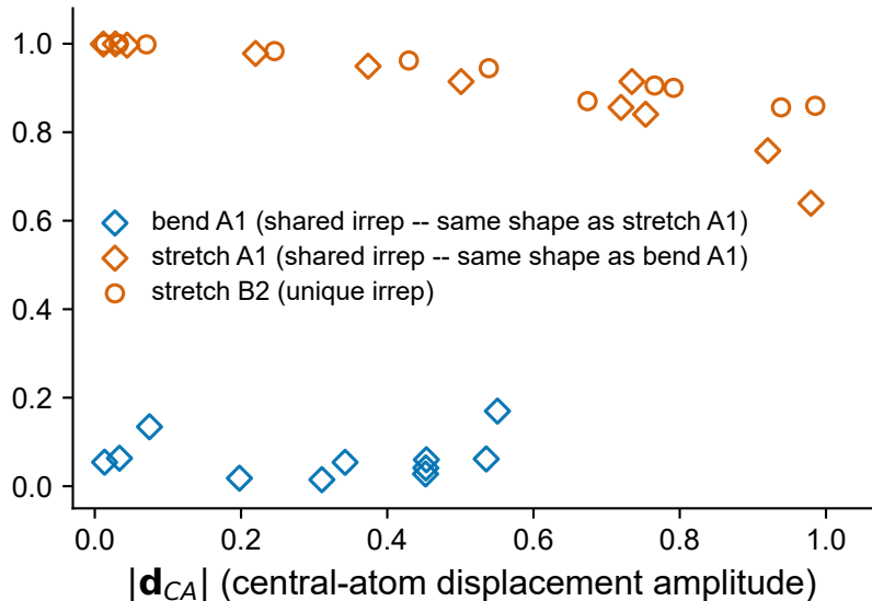
(b) Bent AB 2 (non-ideal)
