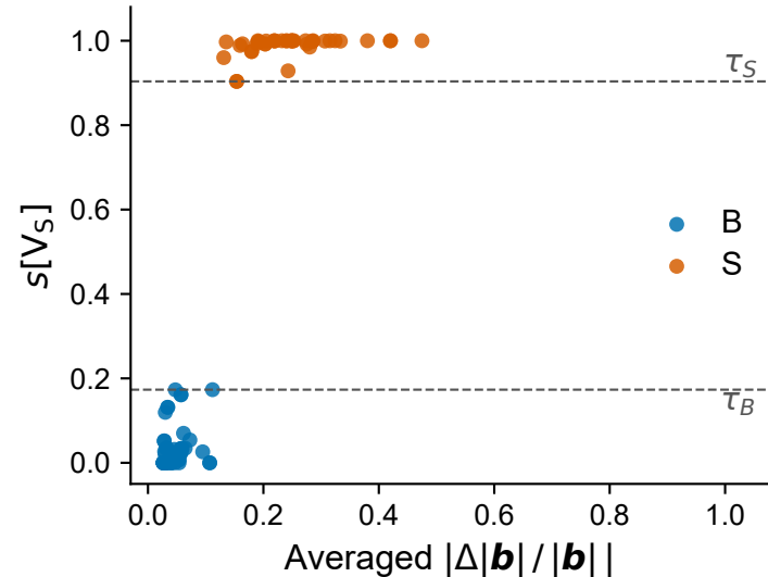
(a) Ideal molecules
