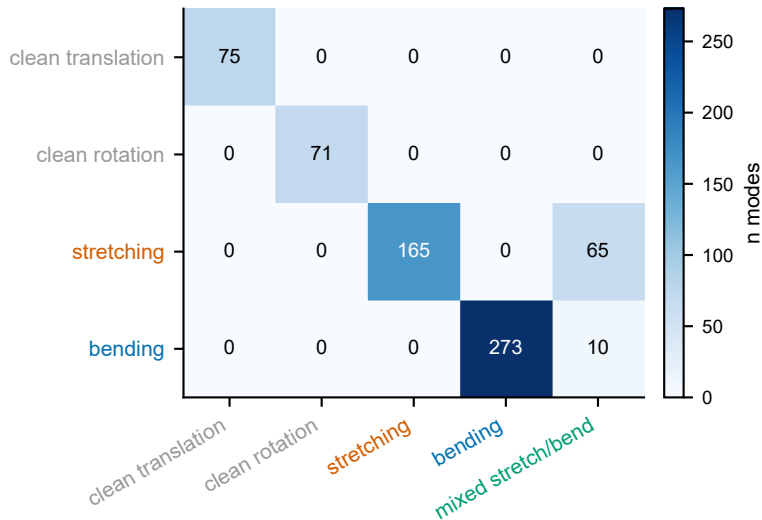
(a) Confusion matrix
