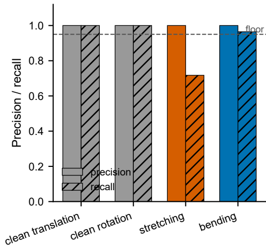
(b) Per-category precision/recall
