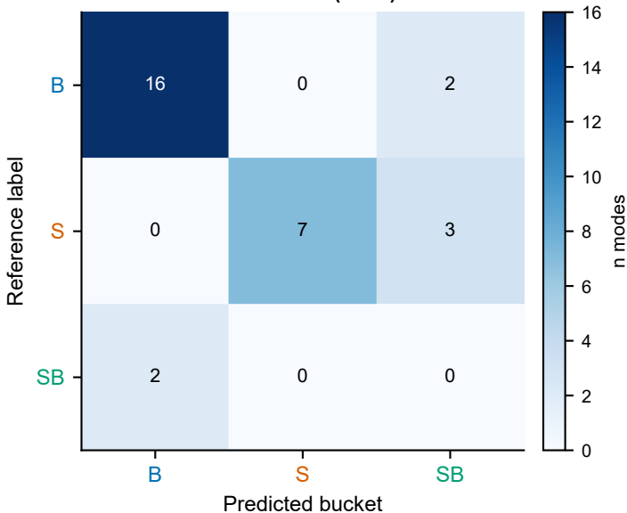
Benzene internal modes (n=30)
