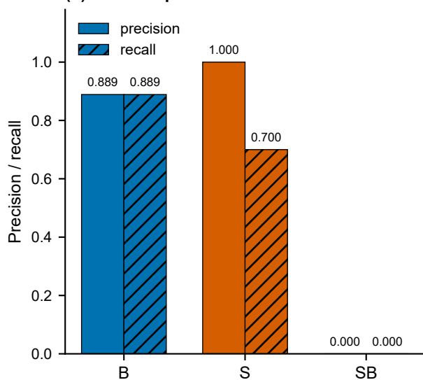
(b) Benzene precision/recall
