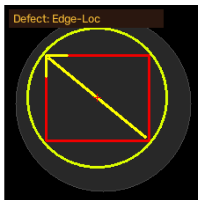
Sample #8: wafer_matrix_sample_08.png Class: Edge-Loc (57.5%) Defect Clusters: 1
