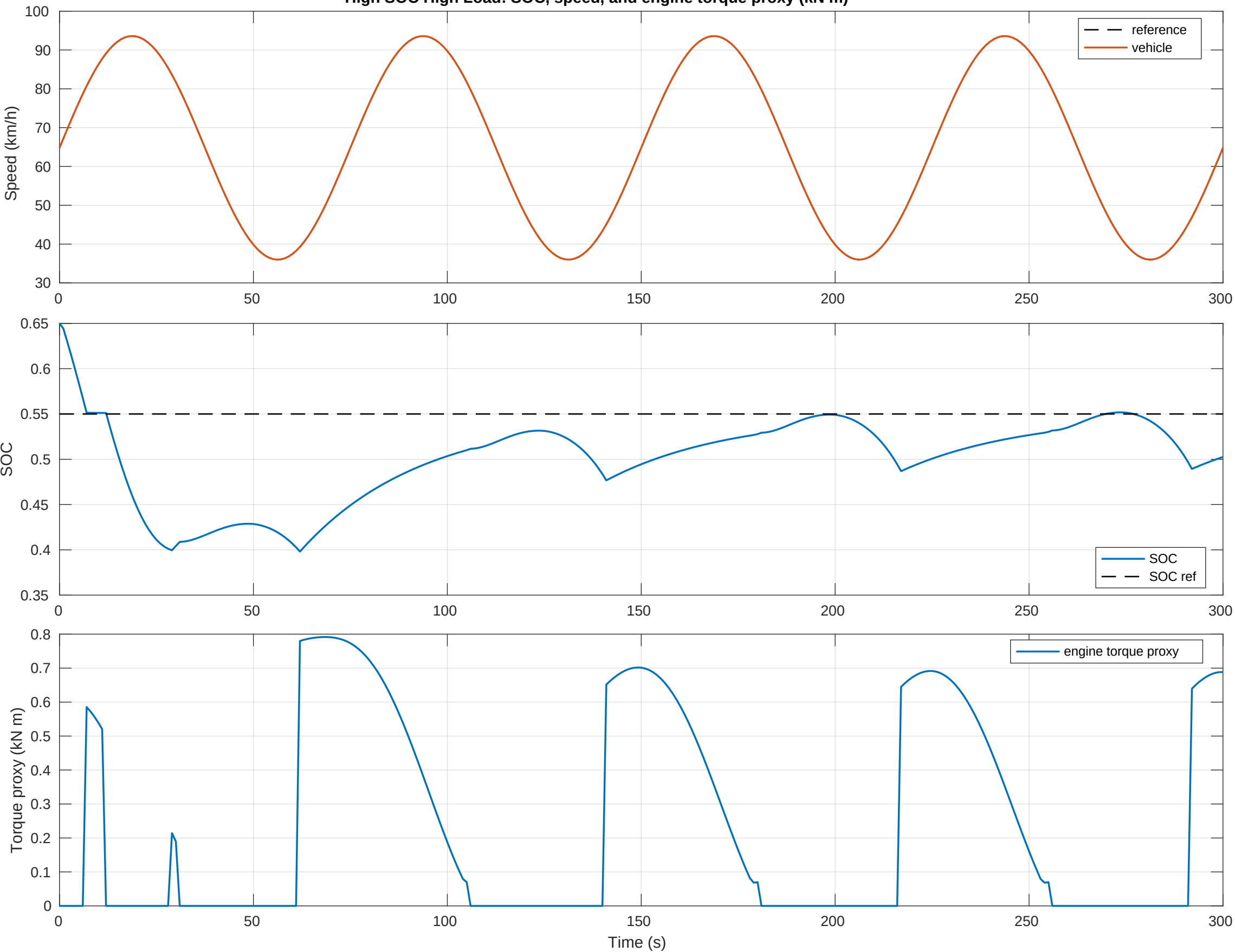
High SOC High Load: SOC, speed, and engine torque proxy (kN m)
