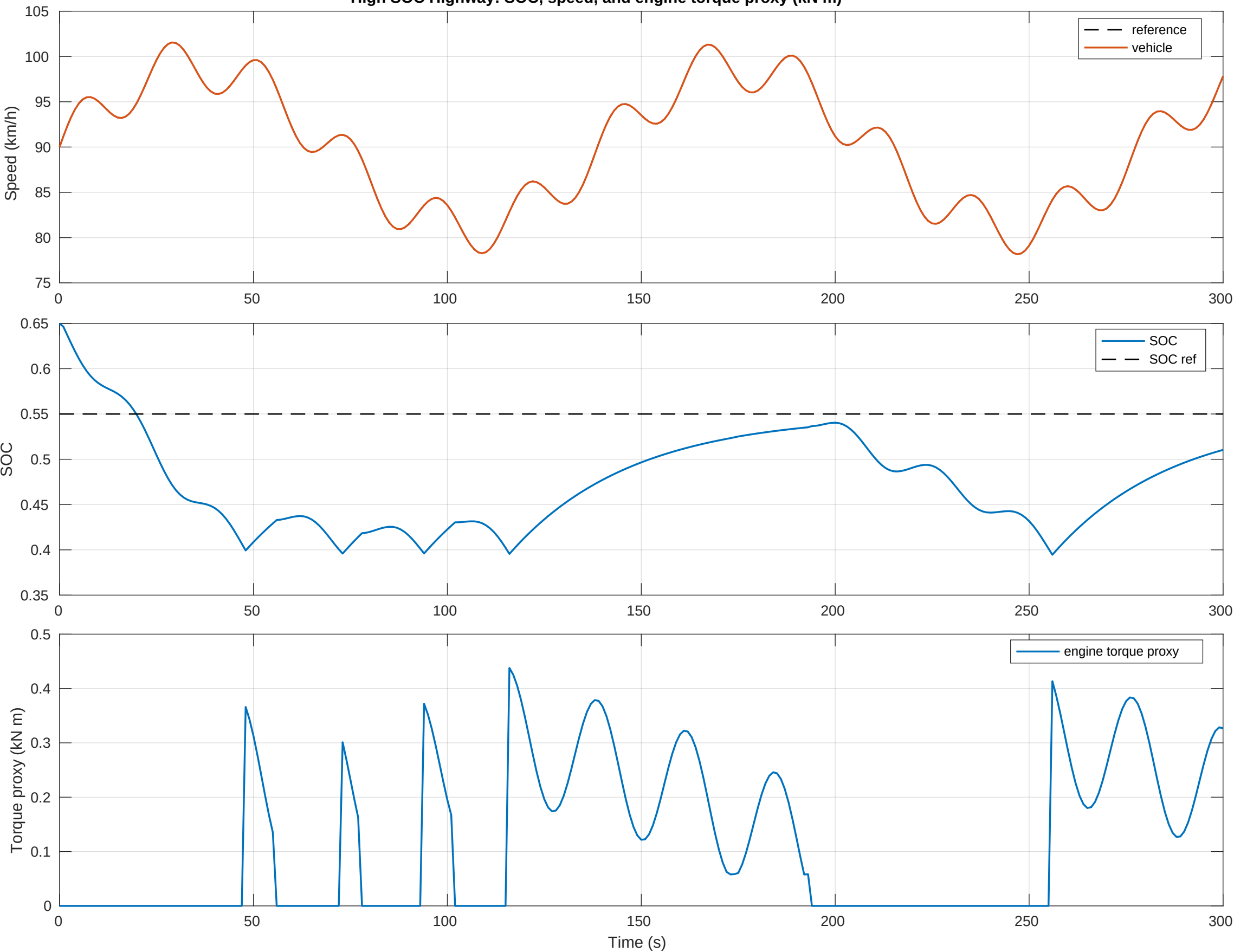
High SOC Highway: SOC, speed, and engine torque proxy (kN m)
