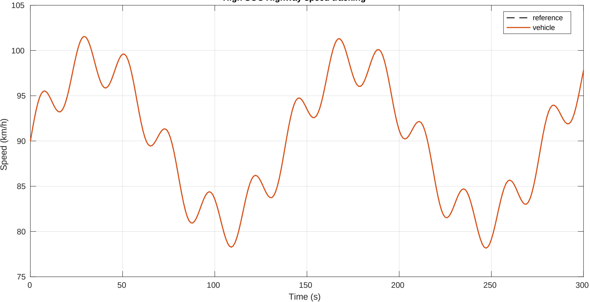
High SOC Highway speed tracking
