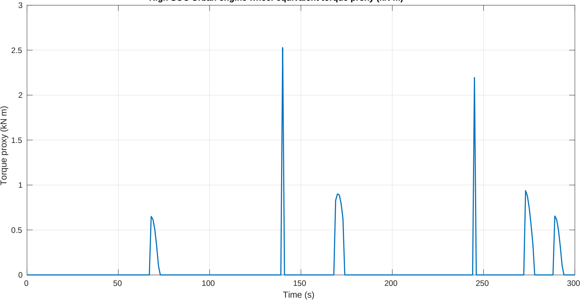
High SOC Urban engine wheel-equivalent torque proxy (kN m)
