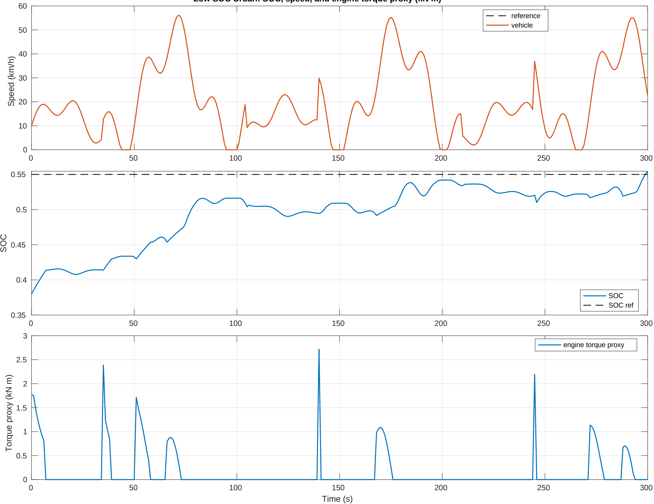
Low SOC Urban: SOC, speed, and engine torque proxy (kN m)
