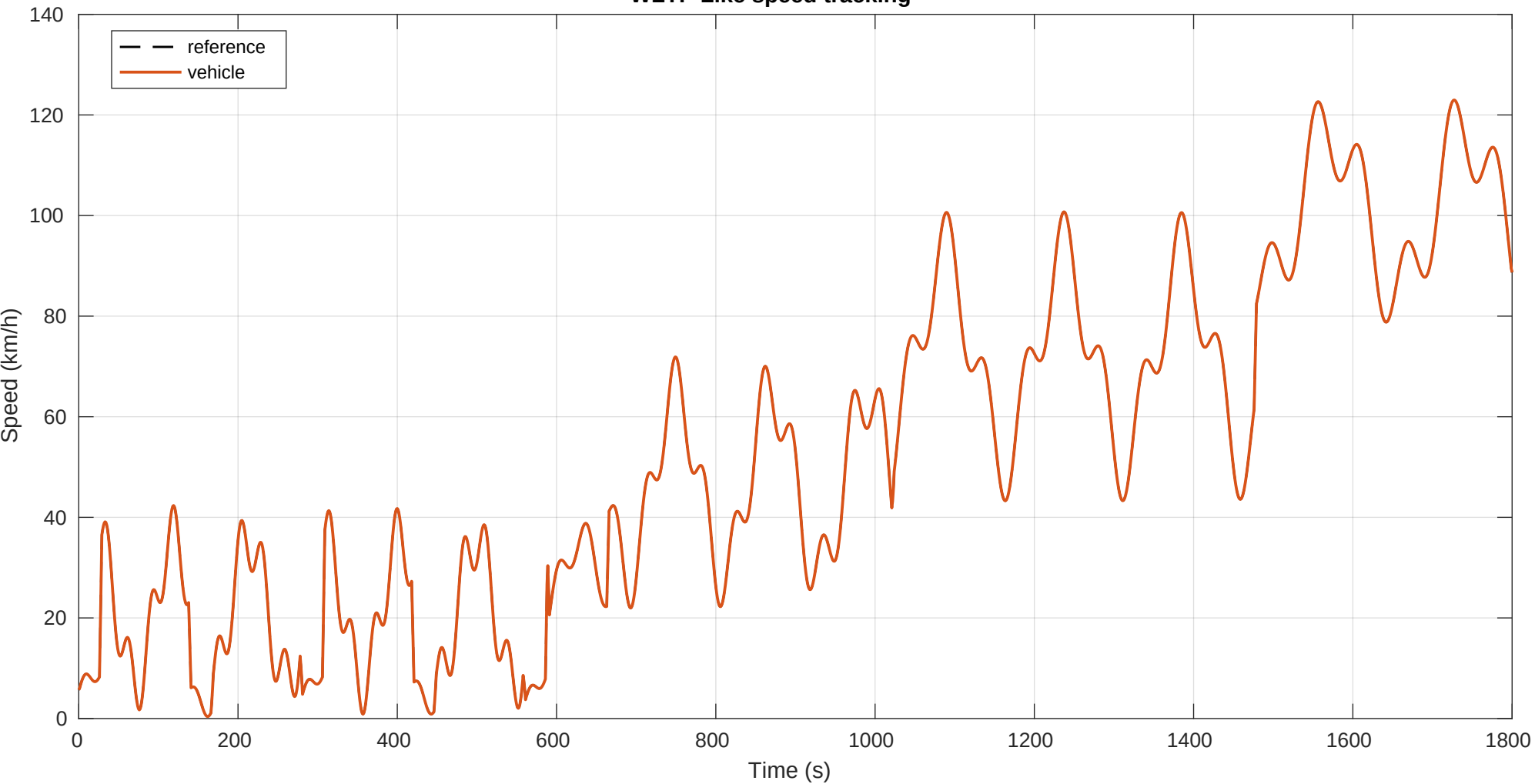
WLTP Like speed tracking
