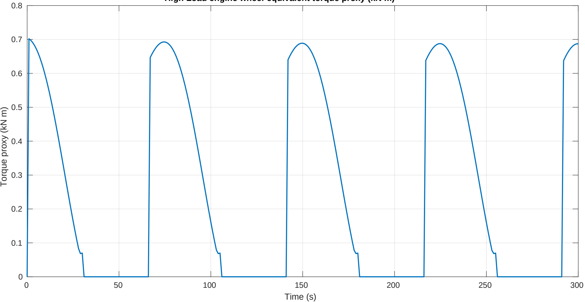
High Load engine wheel-equivalent torque proxy (kN m)
