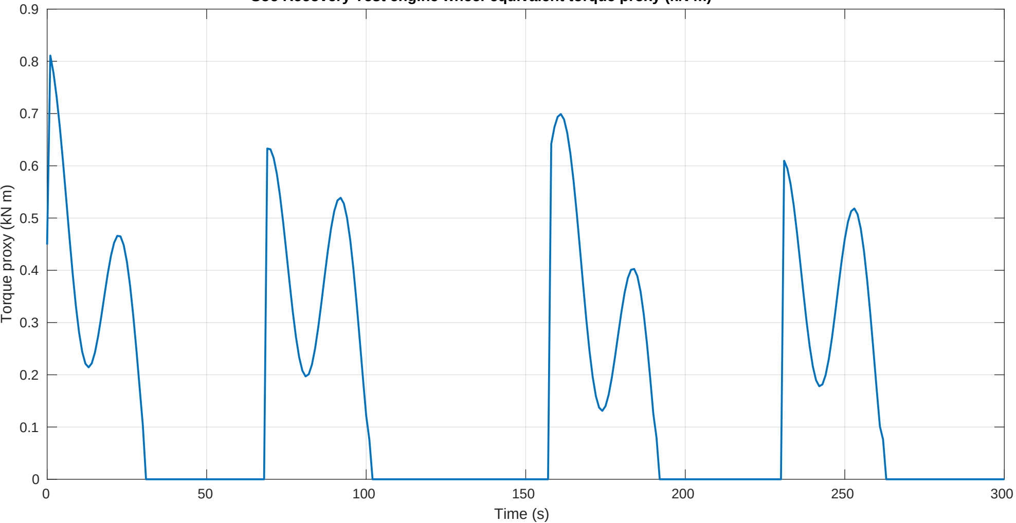
Soc Recovery Test engine wheel-equivalent torque proxy (kN m)
