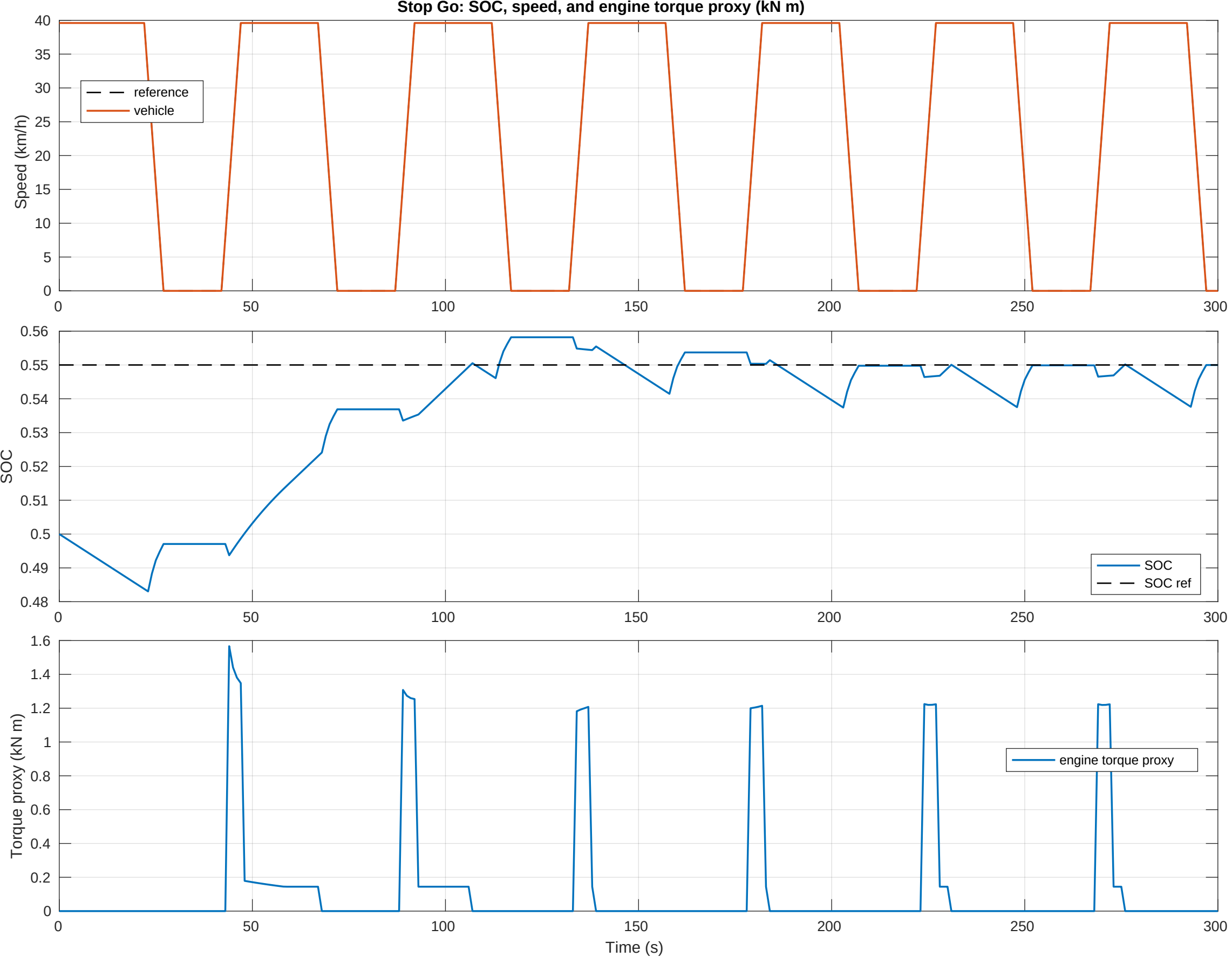
Stop Go: SOC, speed, and engine torque proxy (kN m)
