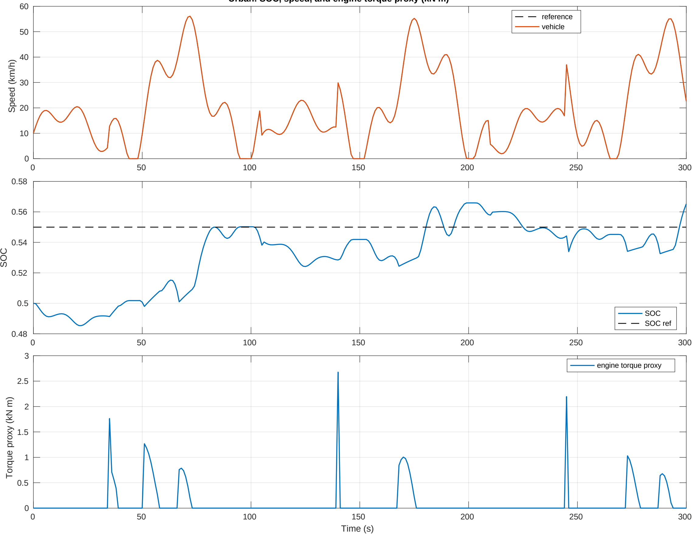
Urban: SOC, speed, and engine torque proxy (kN m)
