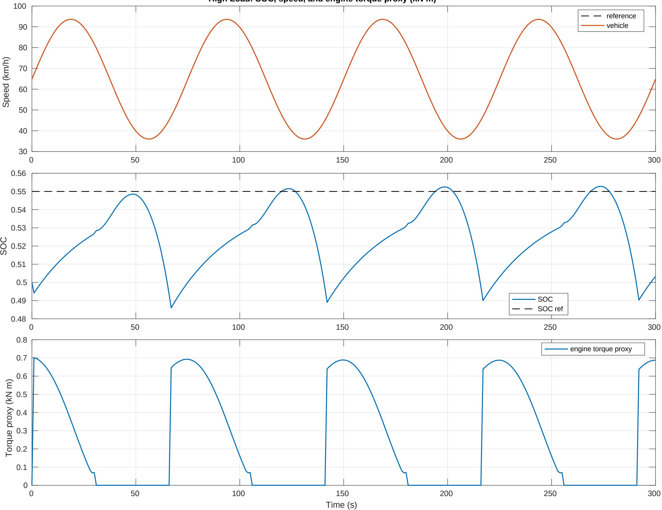
High Load: SOC, speed, and engine torque proxy (kN m)
