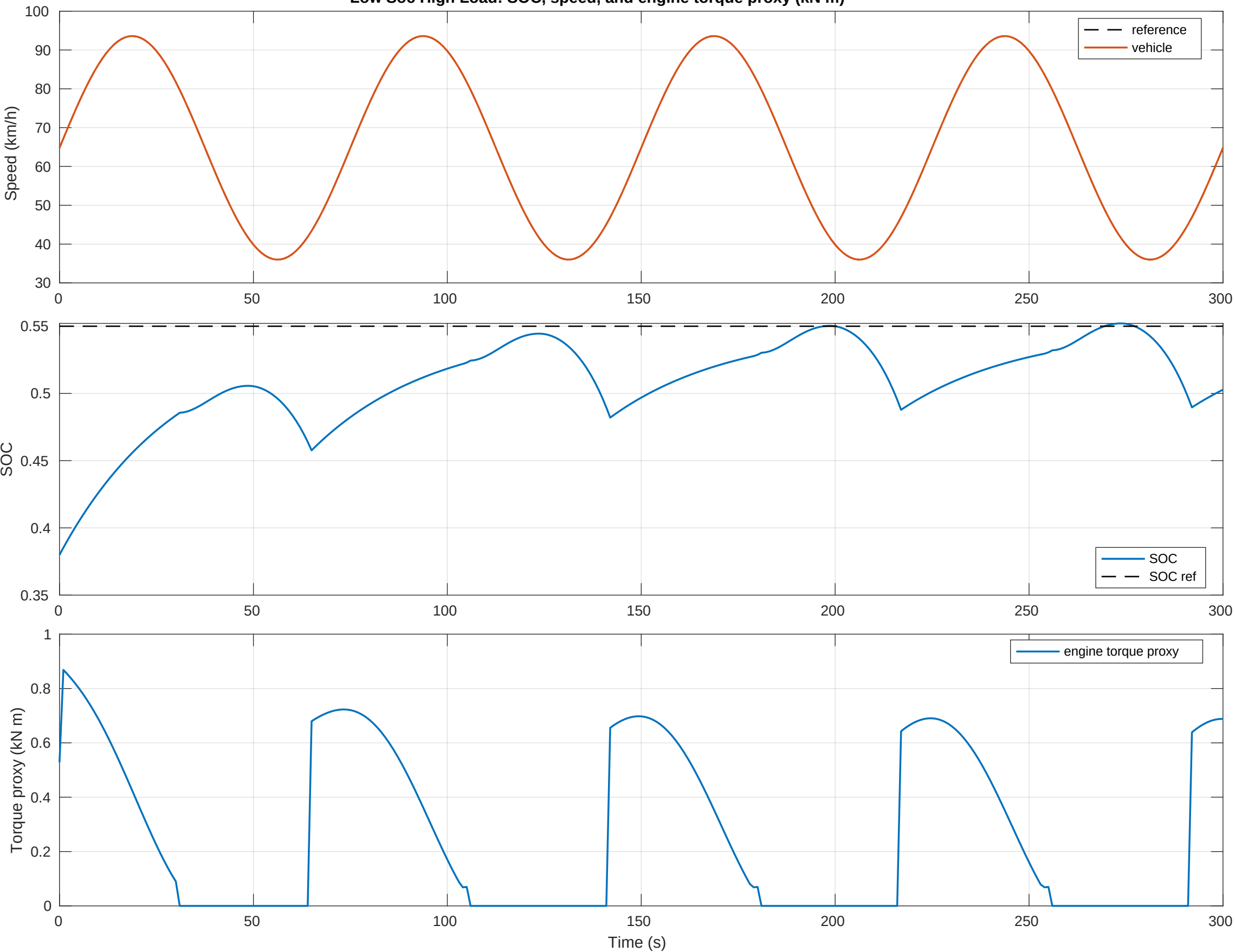
Low Soc High Load: SOC, speed, and engine torque proxy (kN m)
