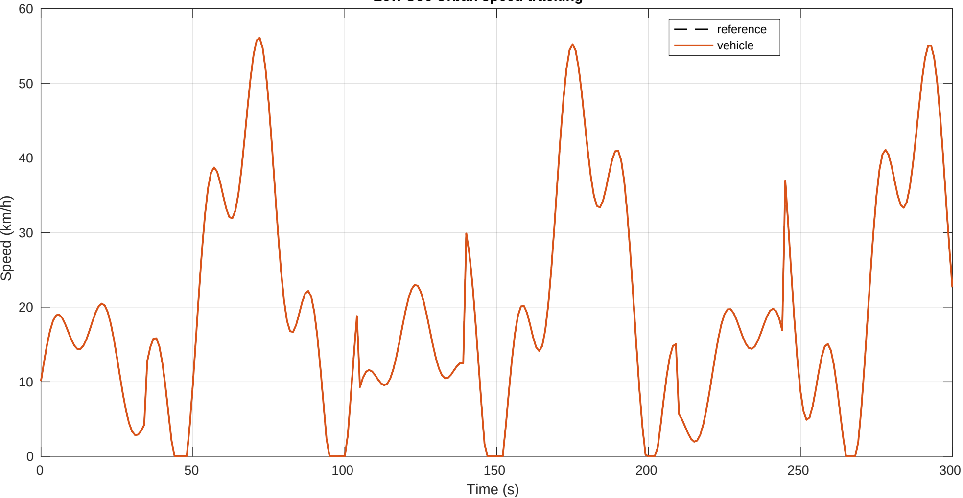
Low Soc Urban speed tracking
