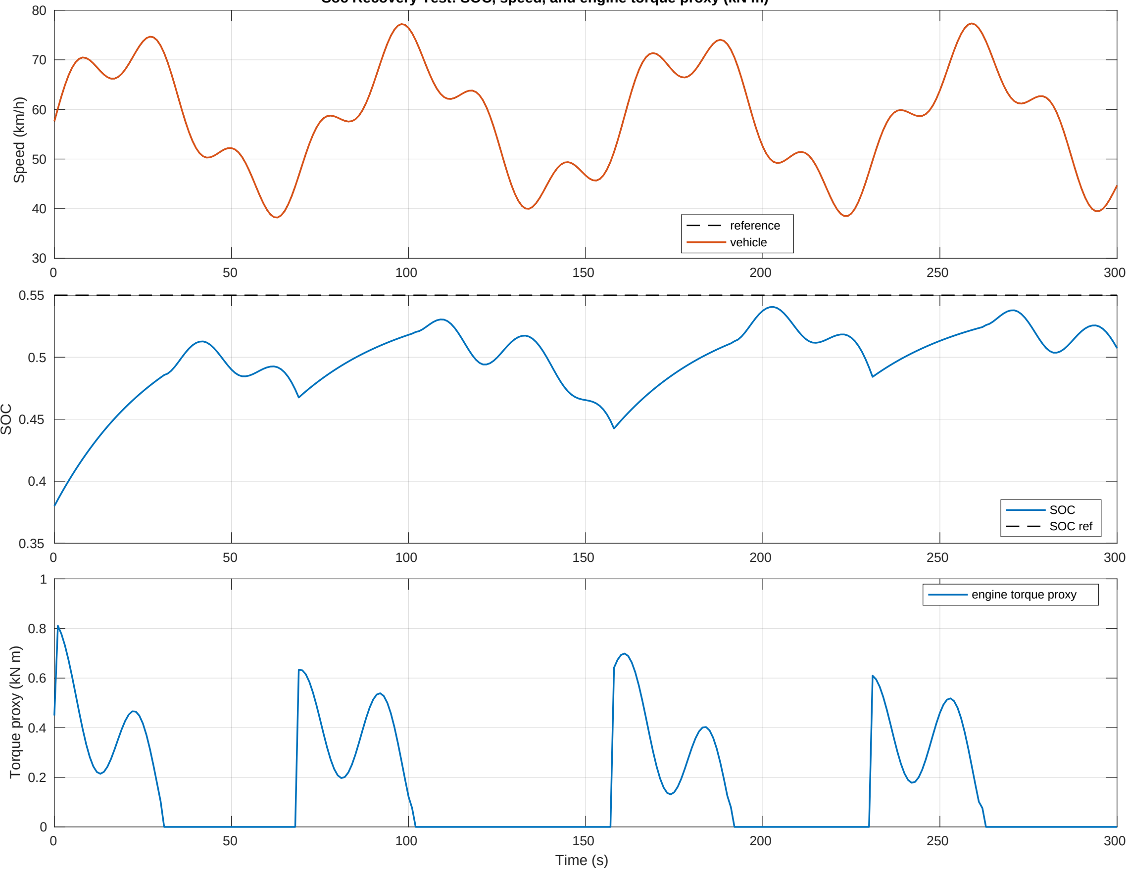
Soc Recovery Test: SOC, speed, and engine torque proxy (kN m)
