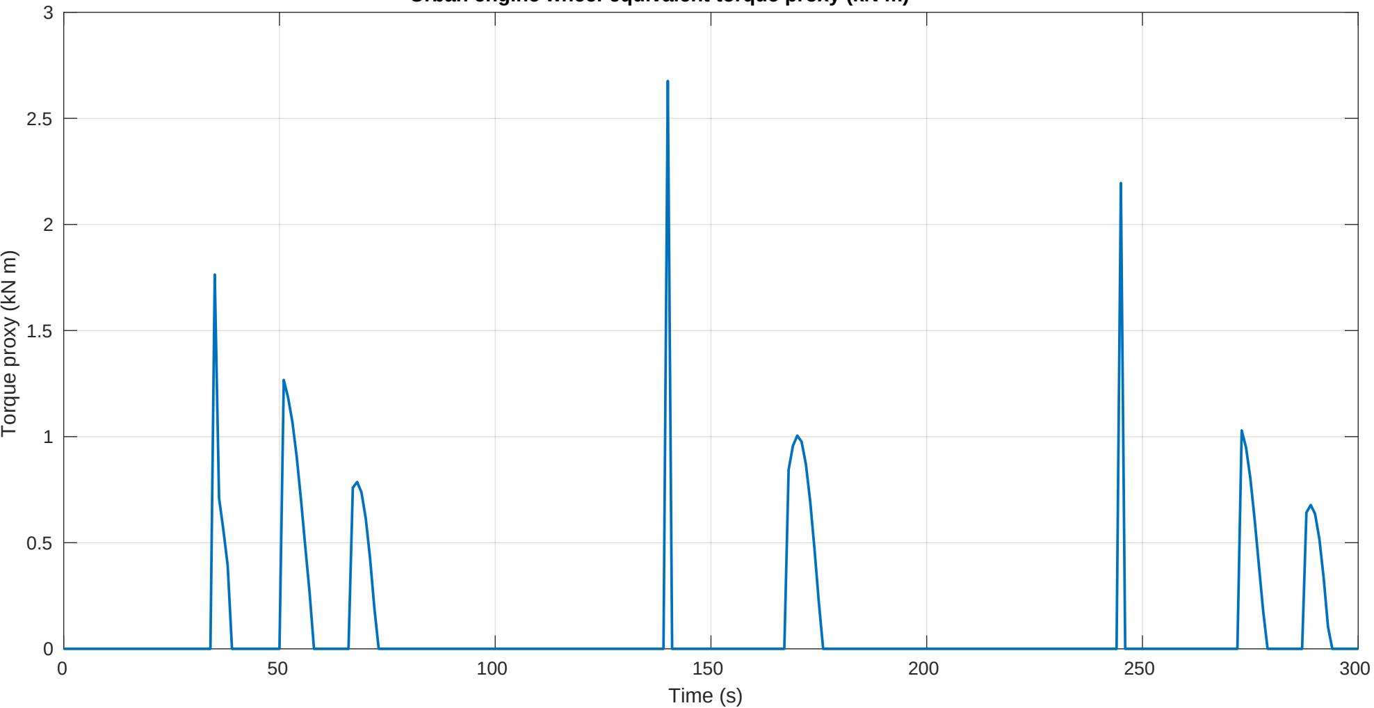
Urban engine wheel-equivalent torque proxy (kN m)
