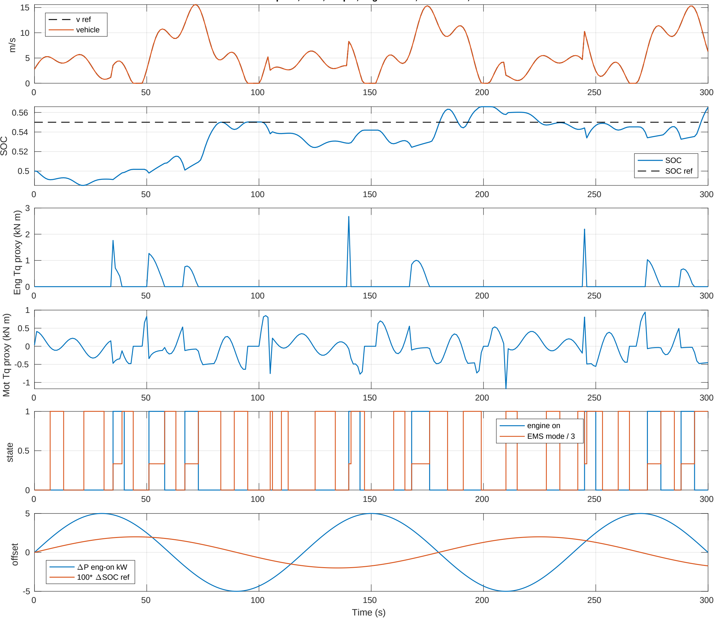
Test Process Trace: speed, SOC, torque, engine state, EMS mode, offsets
