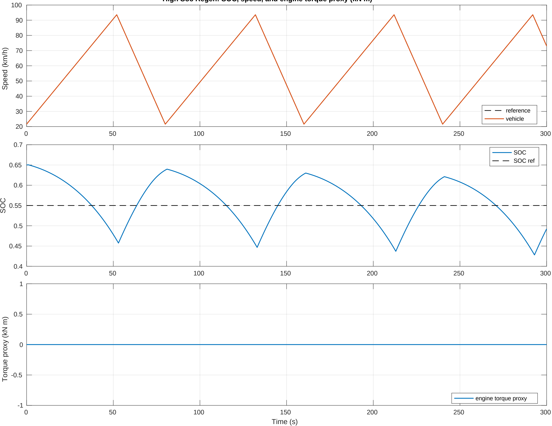
High Soc Regen: SOC, speed, and engine torque proxy (kN m)
