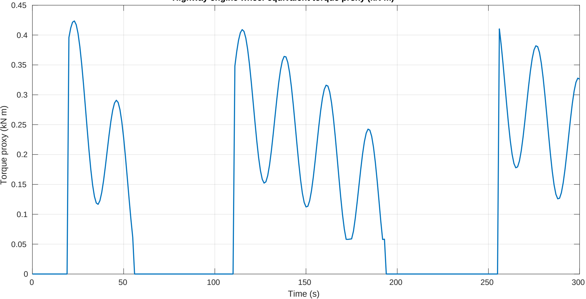
Highway engine wheel-equivalent torque proxy (kN m)
