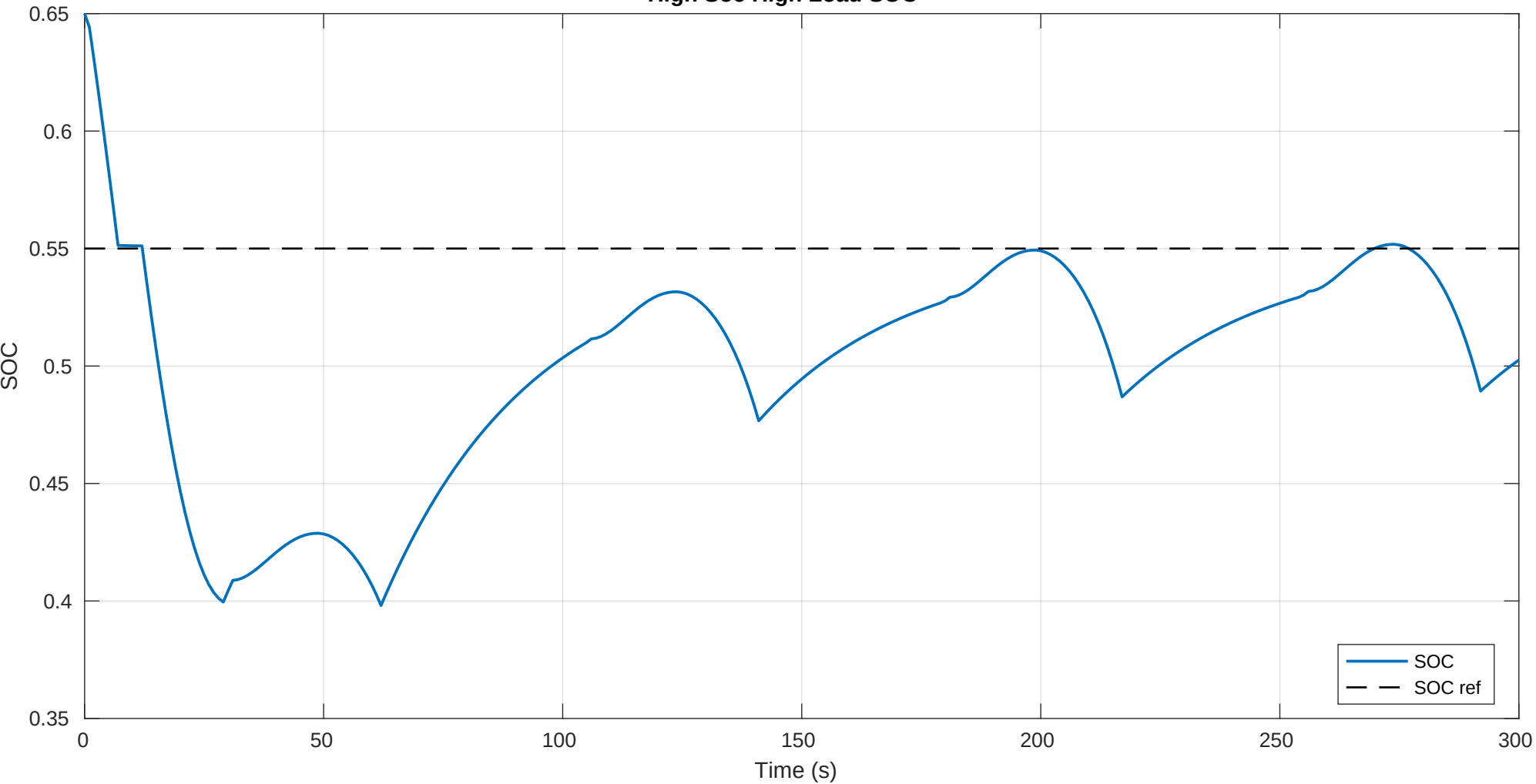
High Soc High Load SOC
