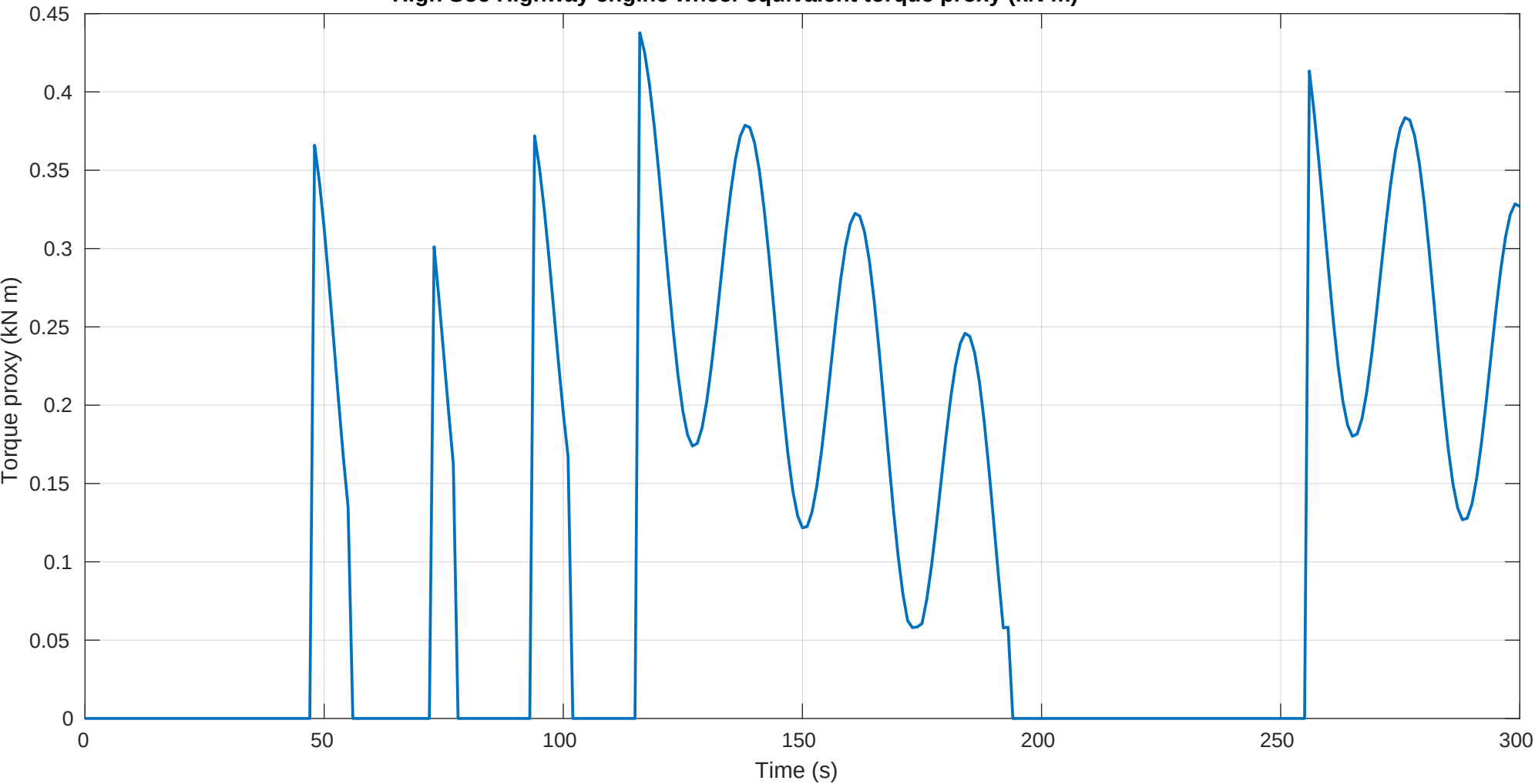
High Soc Highway engine wheel-equivalent torque proxy (kN m)
