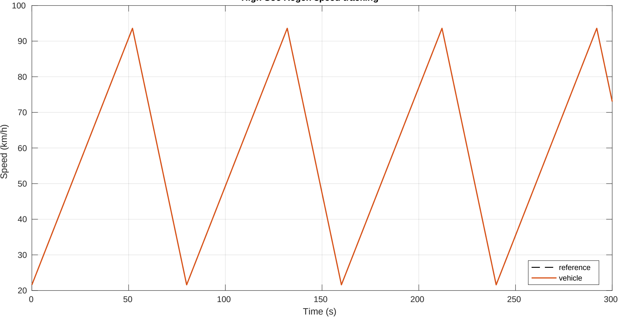
High Soc Regen speed tracking
