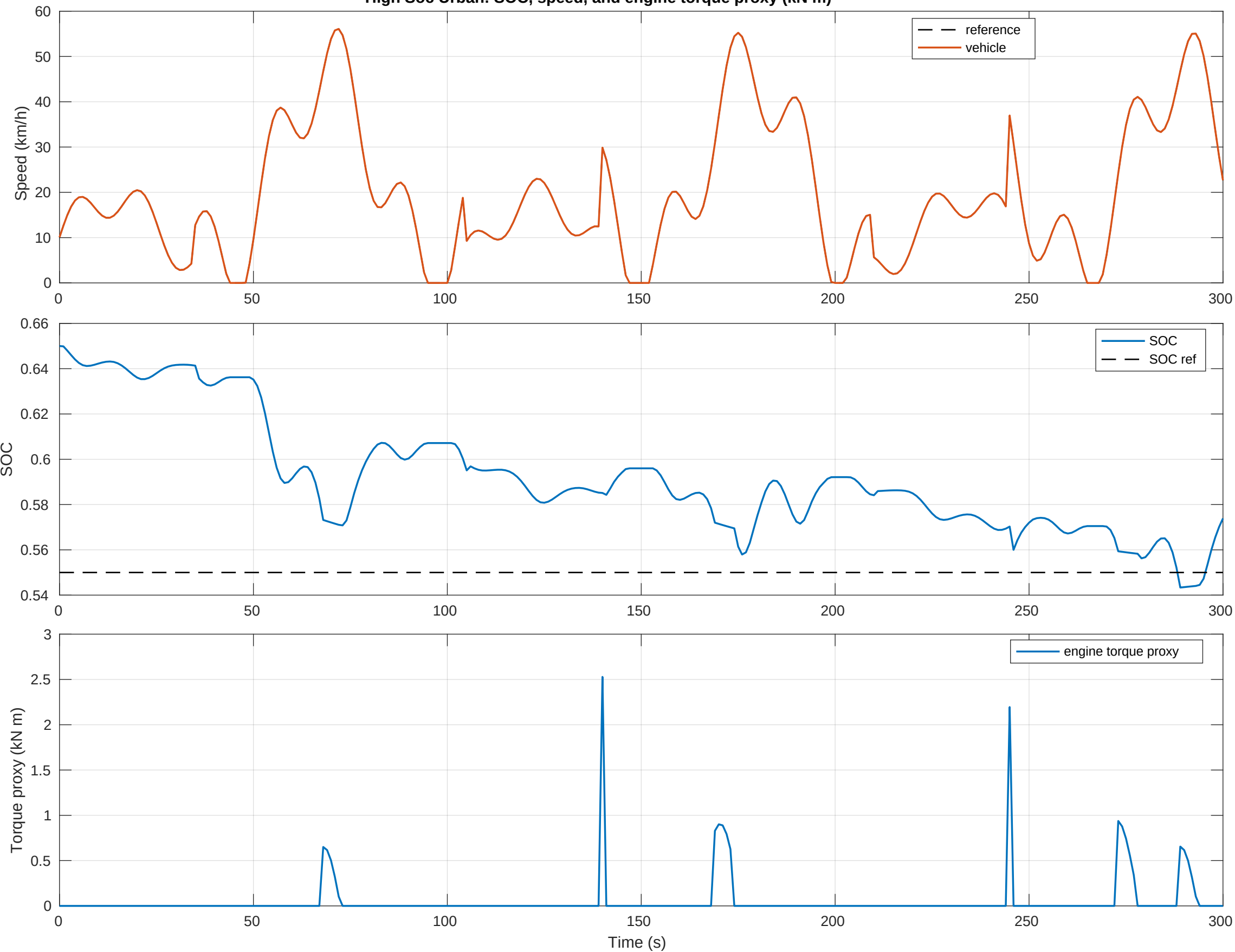
High Soc Urban: SOC, speed, and engine torque proxy (kN m)
