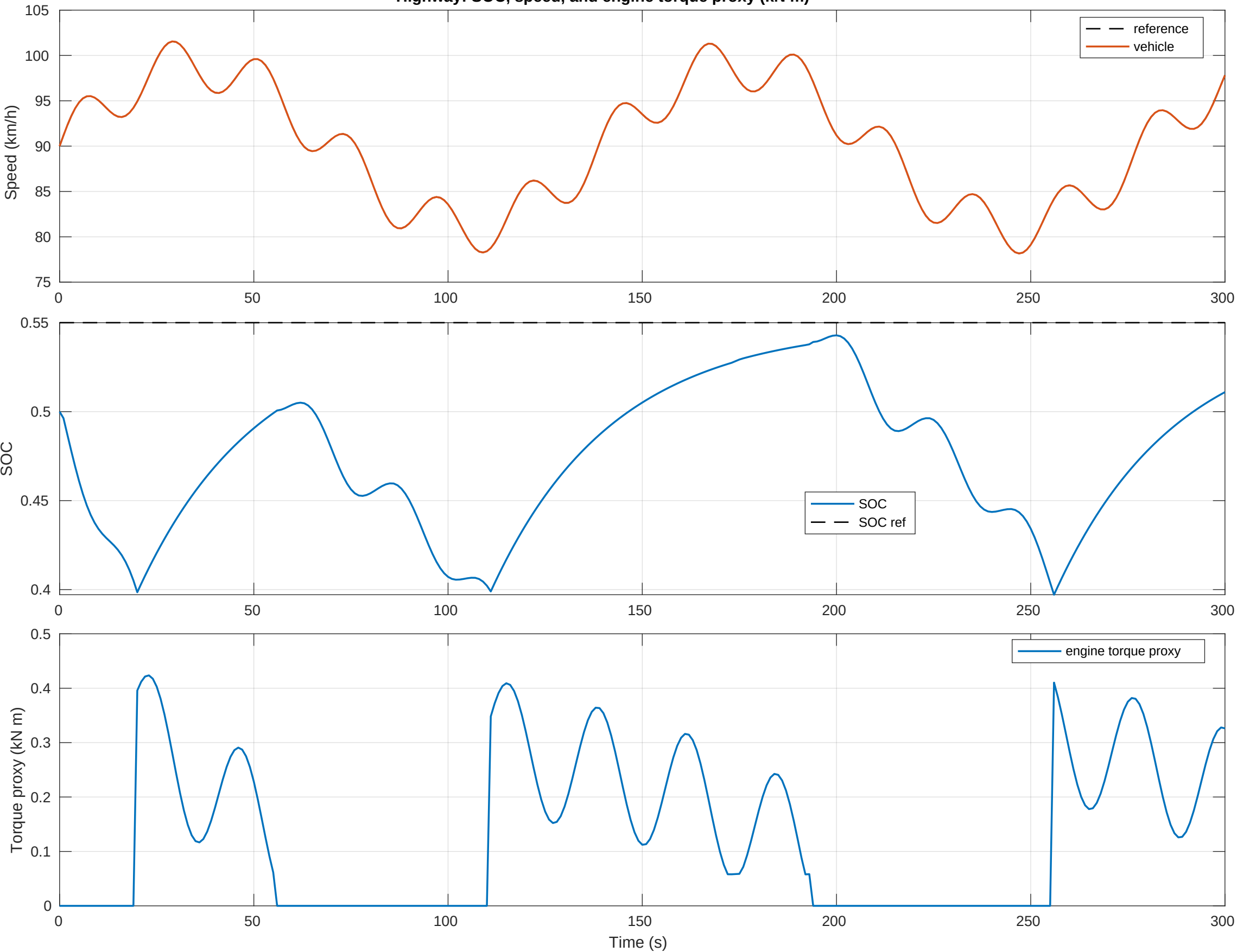
Highway: SOC, speed, and engine torque proxy (kN m)
