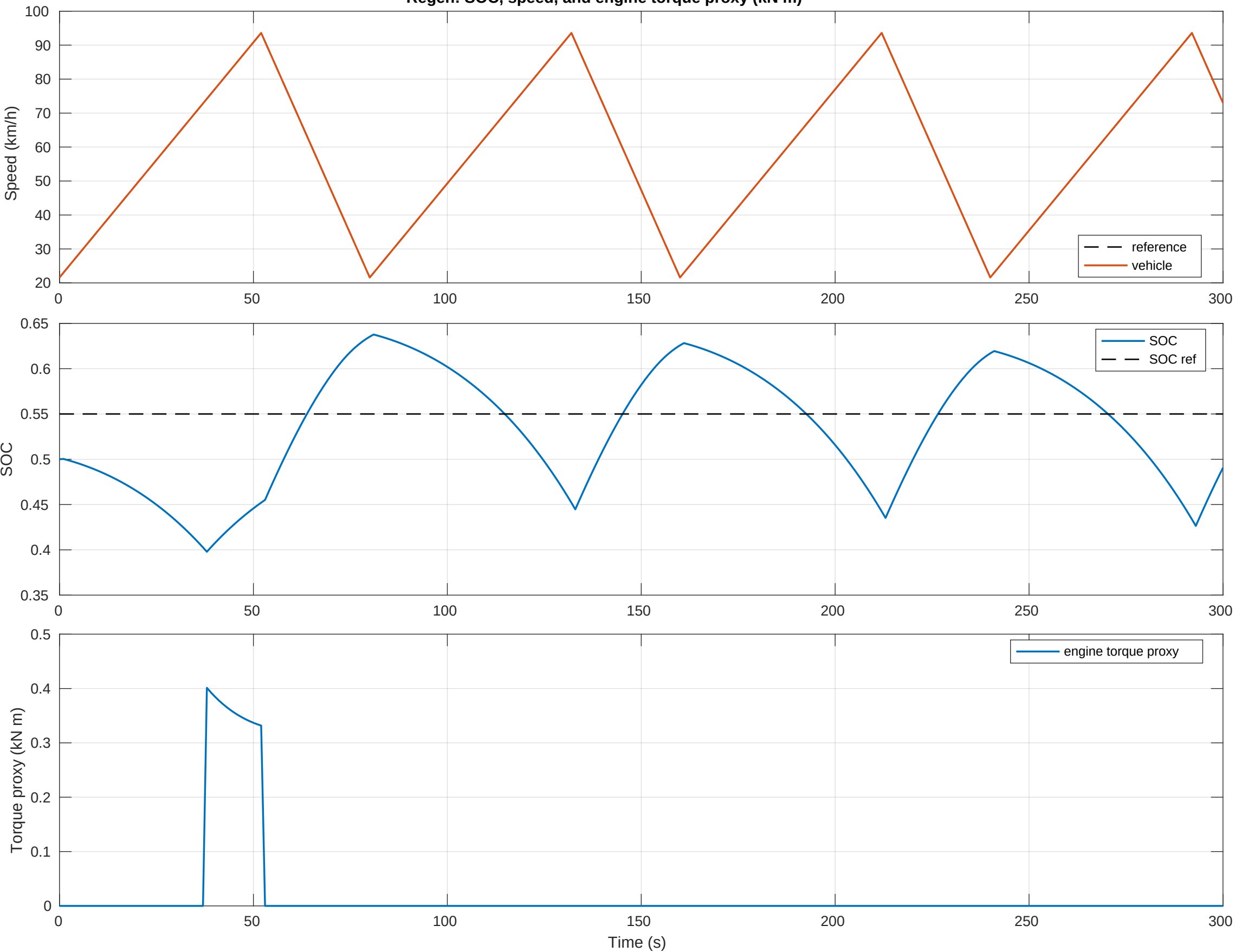
Regen: SOC, speed, and engine torque proxy (kN m)
