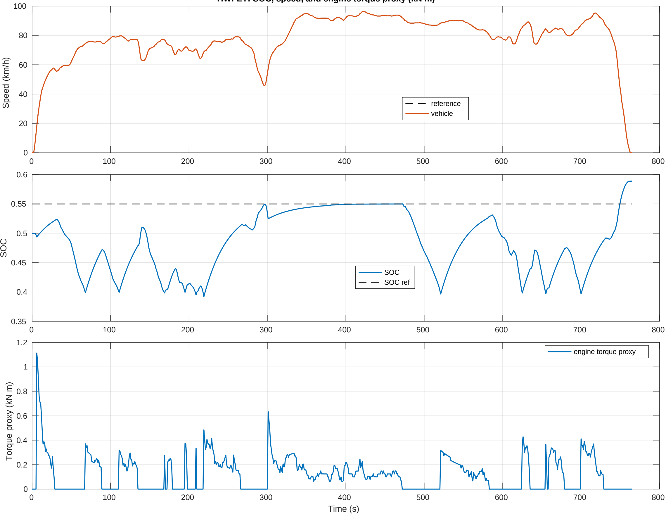
HWFET: SOC, speed, and engine torque proxy (kN m)
