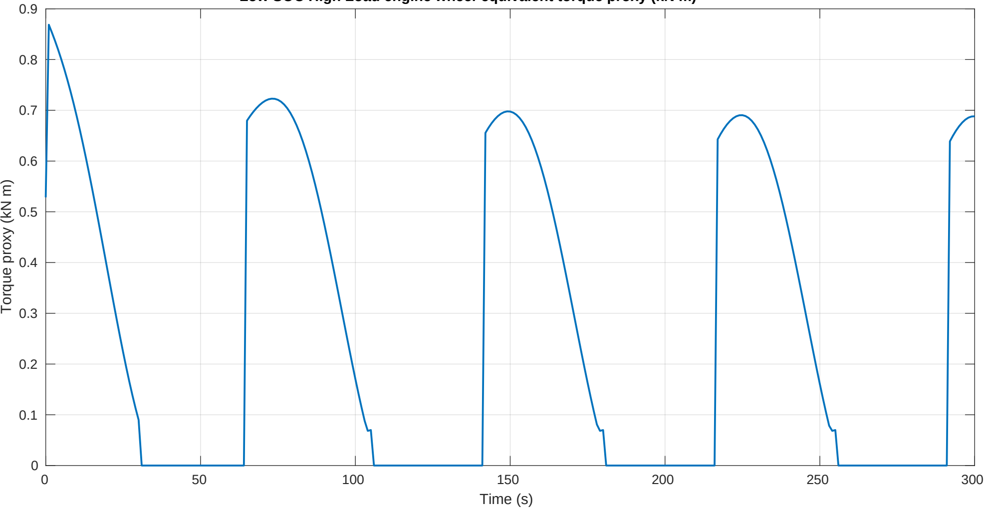
Low SOC High Load engine wheel-equivalent torque proxy (kN m)
