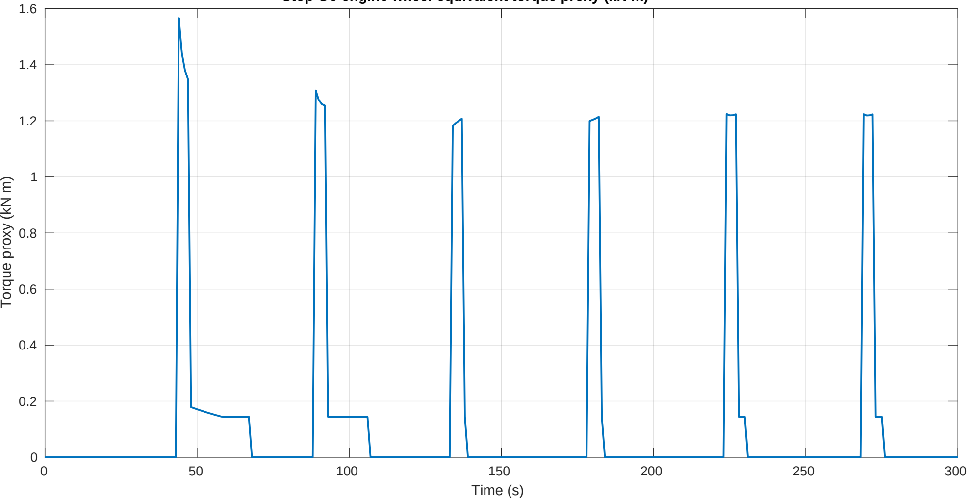
Stop Go engine wheel-equivalent torque proxy (kN m)
