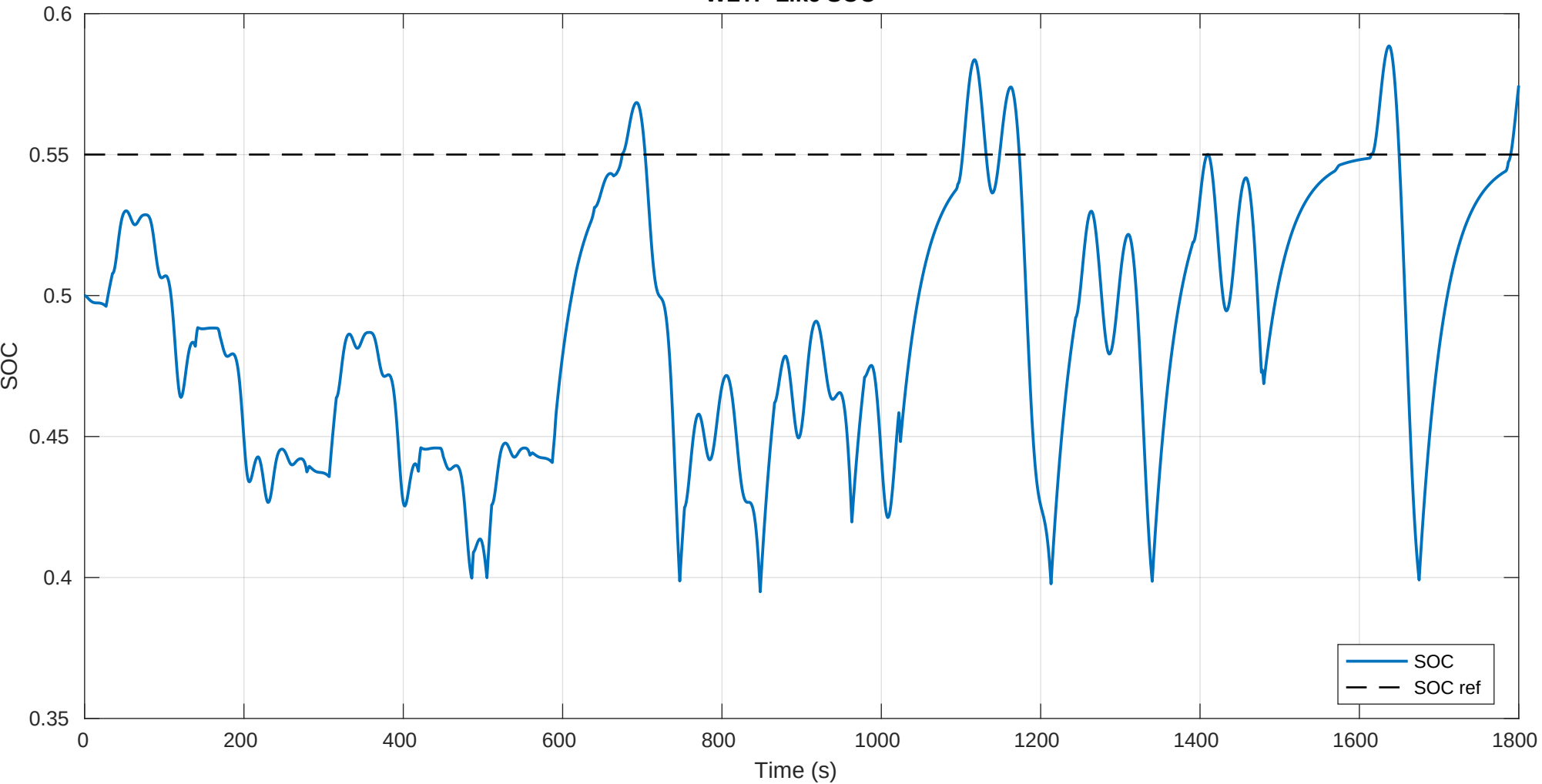
WLTP Like SOC
