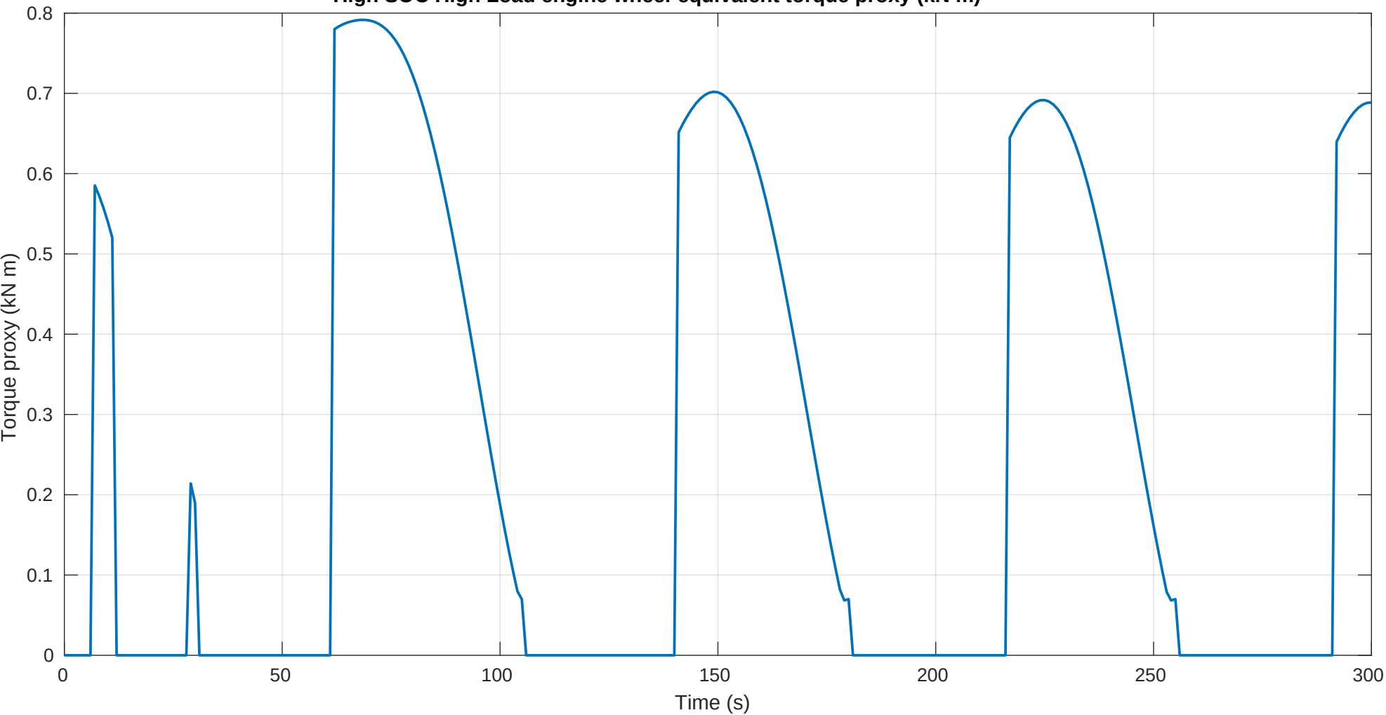
High SOC High Load engine wheel-equivalent torque proxy (kN m)
