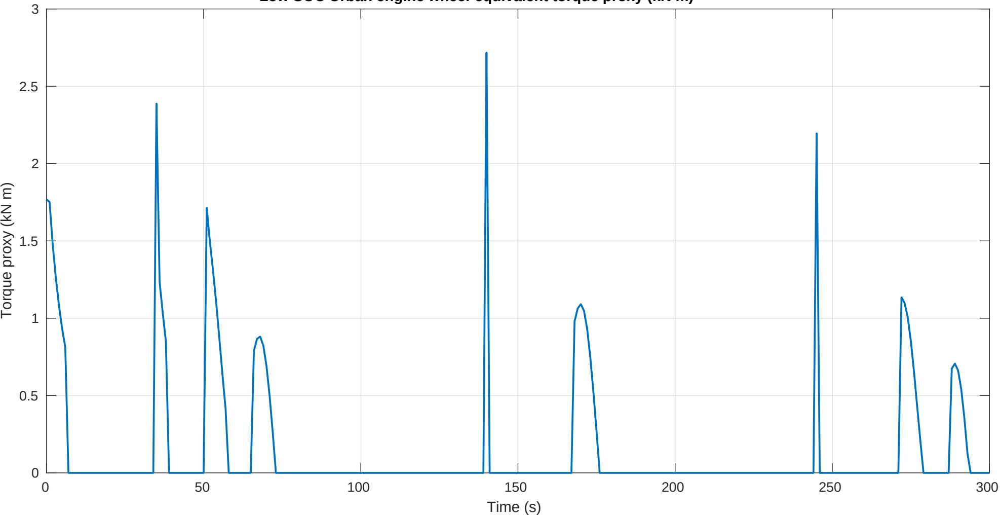
Low SOC Urban engine wheel-equivalent torque proxy (kN m)
