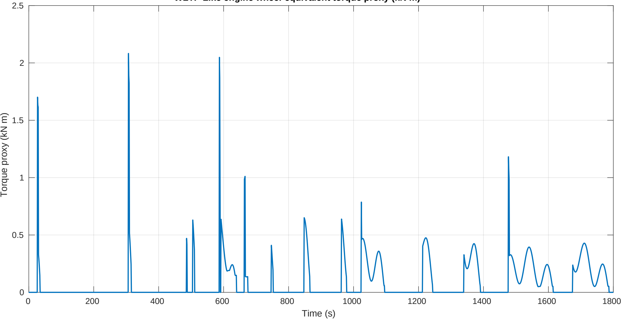
WLTP Like engine wheel-equivalent torque proxy (kN m)
