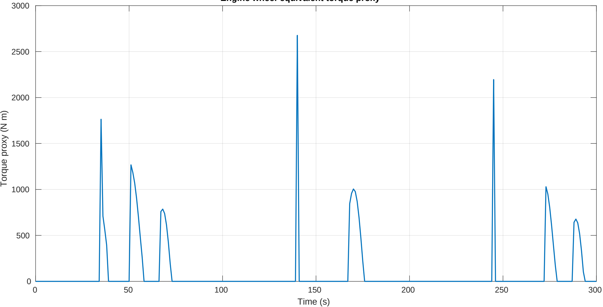
Engine wheel-equivalent torque proxy
