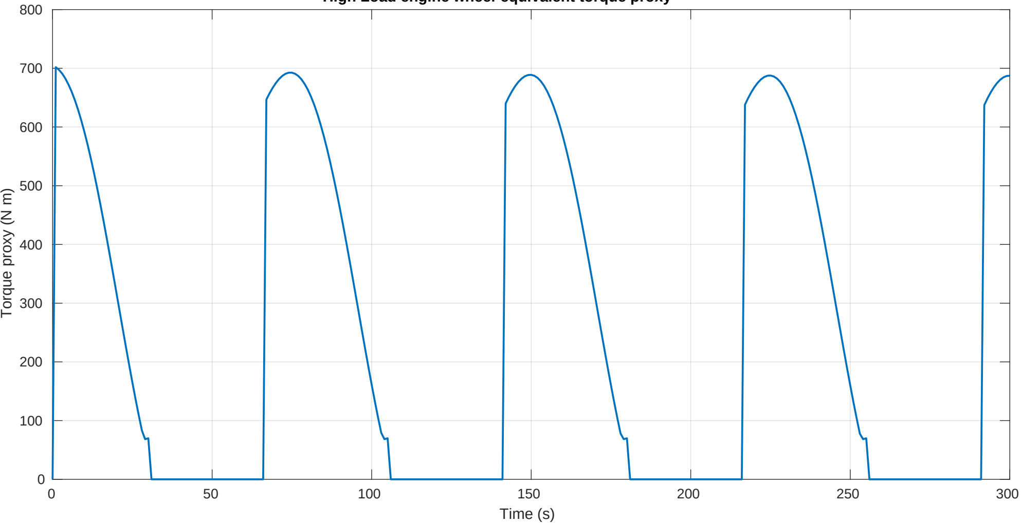
High Load engine wheel-equivalent torque proxy
