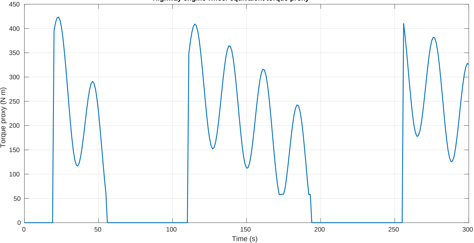
Highway engine wheel-equivalent torque proxy
