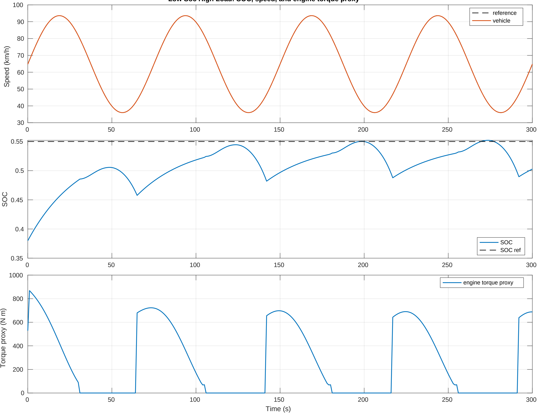
Low Soc High Load: SOC, speed, and engine torque proxy
