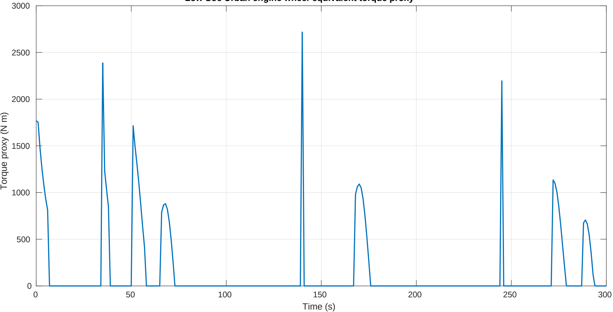
Low Soc Urban engine wheel-equivalent torque proxy
