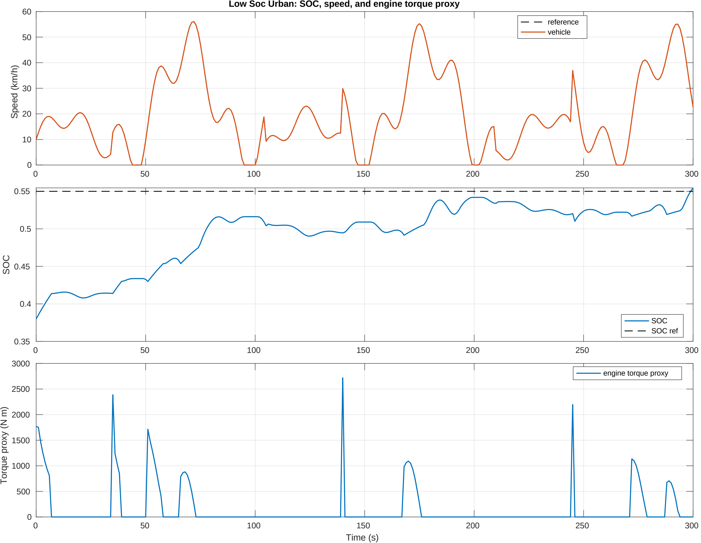
Low Soc Urban: SOC, speed, and engine torque proxy
