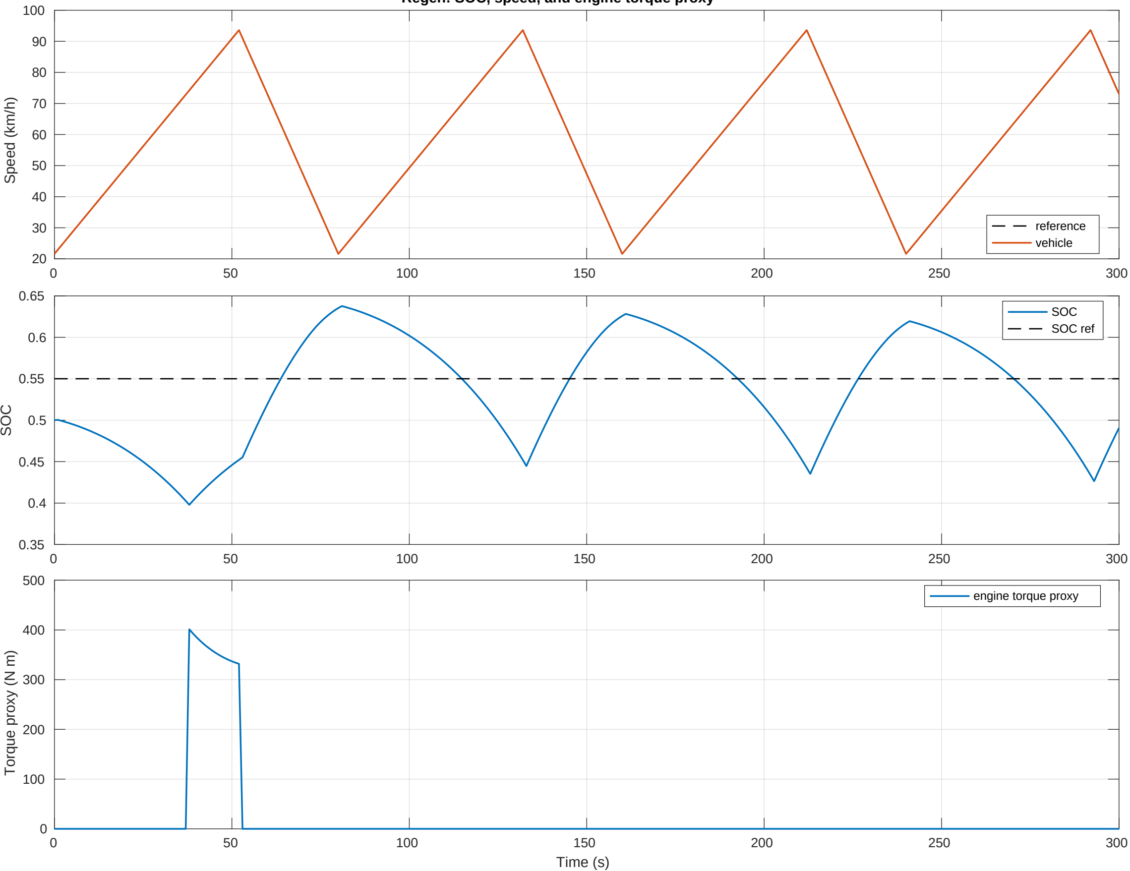
Regen: SOC, speed, and engine torque proxy
